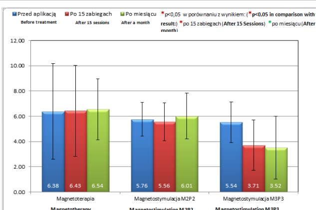
Figure 4: Testosterone concentrations in ng/dl as the mean value and standard deviation before the treatment, after 15 sessions and a month after the end of treatment.
